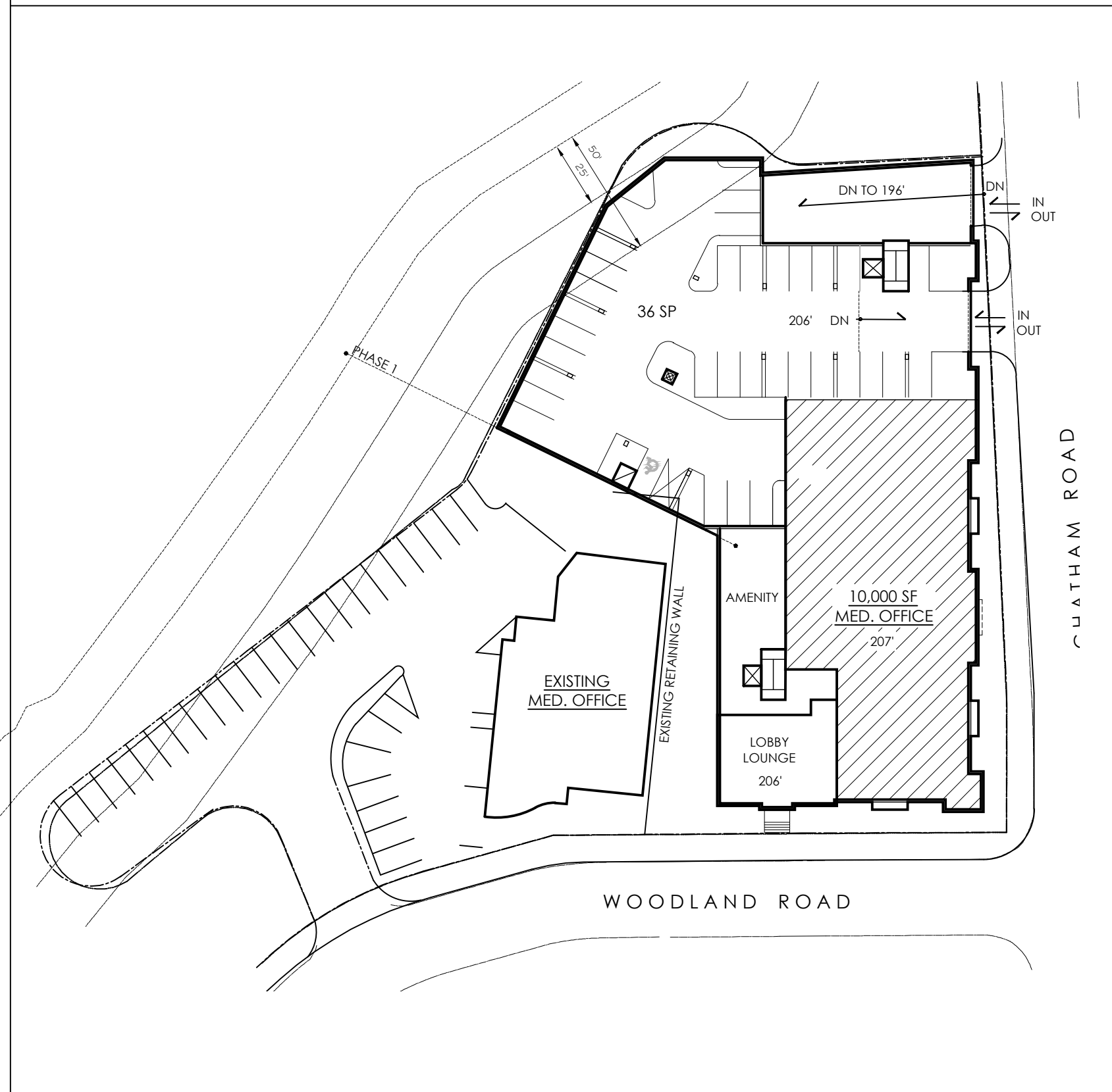
PLAN @ 206', 207'
