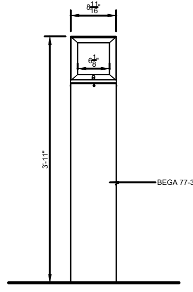
BEGA 77-342 Bollard Not To Scale
