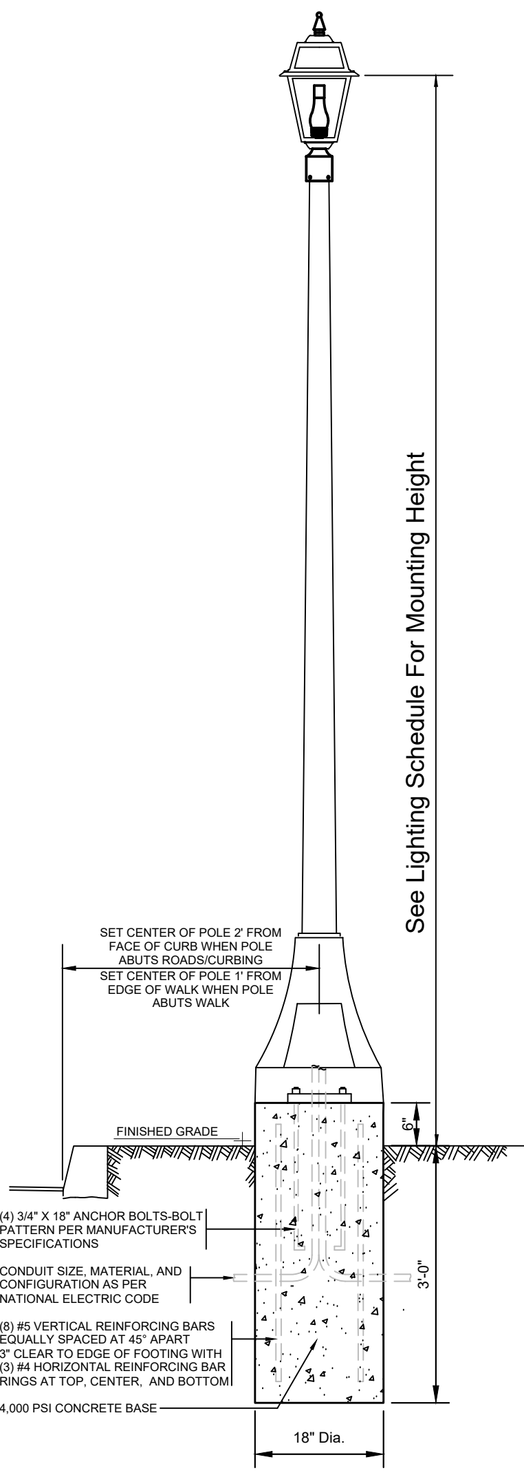
Sternberg 'SEVILLE 440' Luminaire On Smooth Tapered Lancaster Pole Not To Scale
