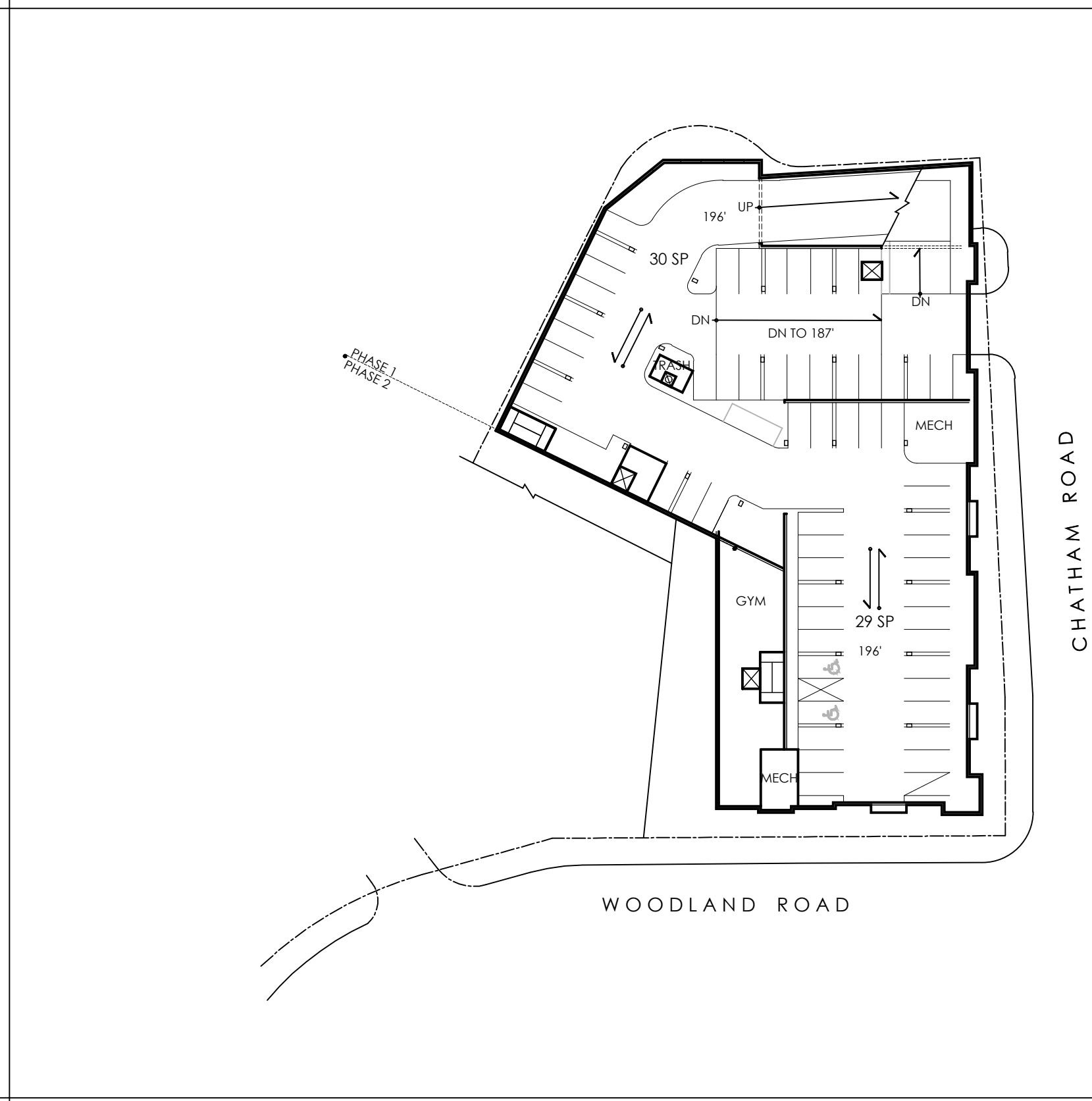
PLAN @ 196', 197'
