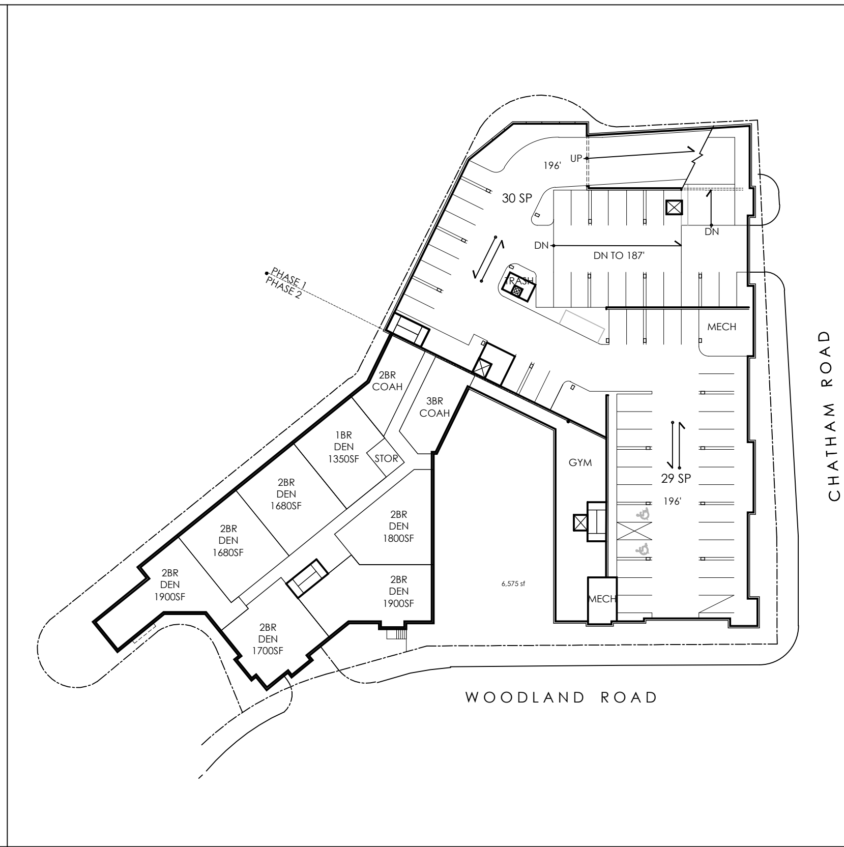
PLAN @ 196', 197'
