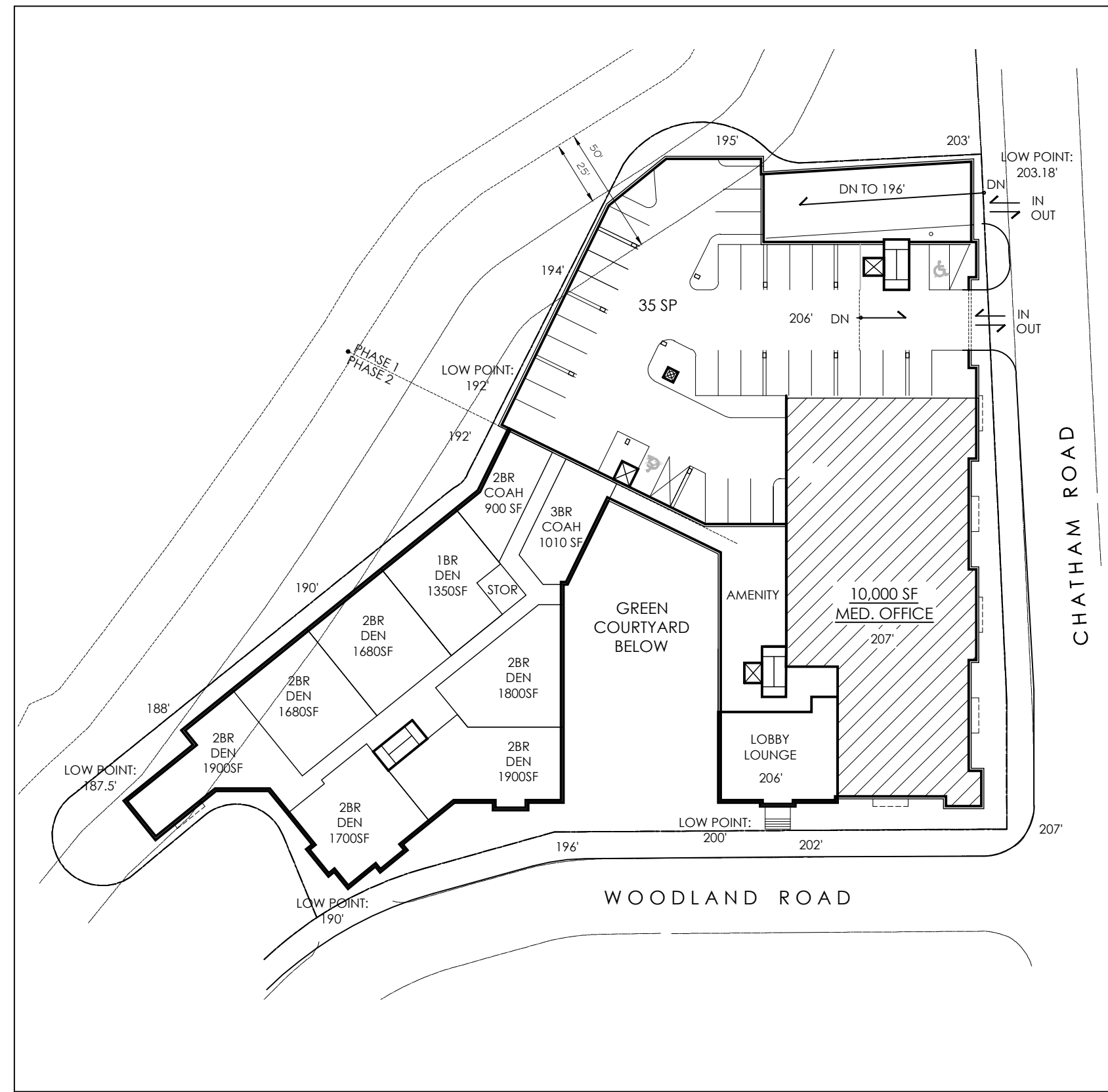
PLAN @ 206', 207'
